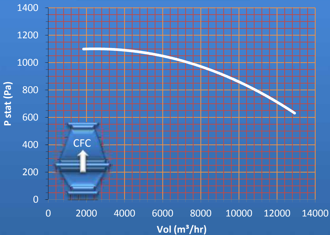
CIV500/500 Performance Curve Motor 11.0kW 1440rpm
