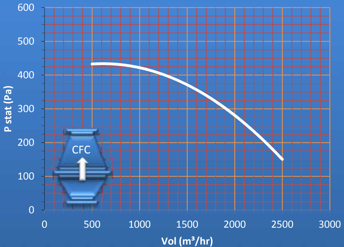
CIV250/250 Performance Curve Motor 0.75kW 1410rpm
