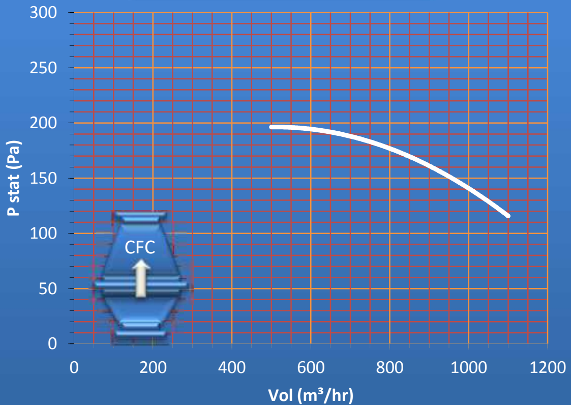
CIV250/200 Performance Curve Motor 0.37kW 1400rpm
