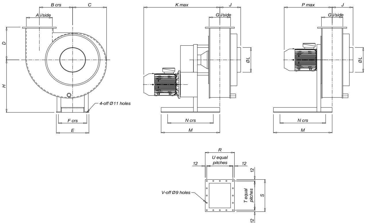
DIMENSION CHART
