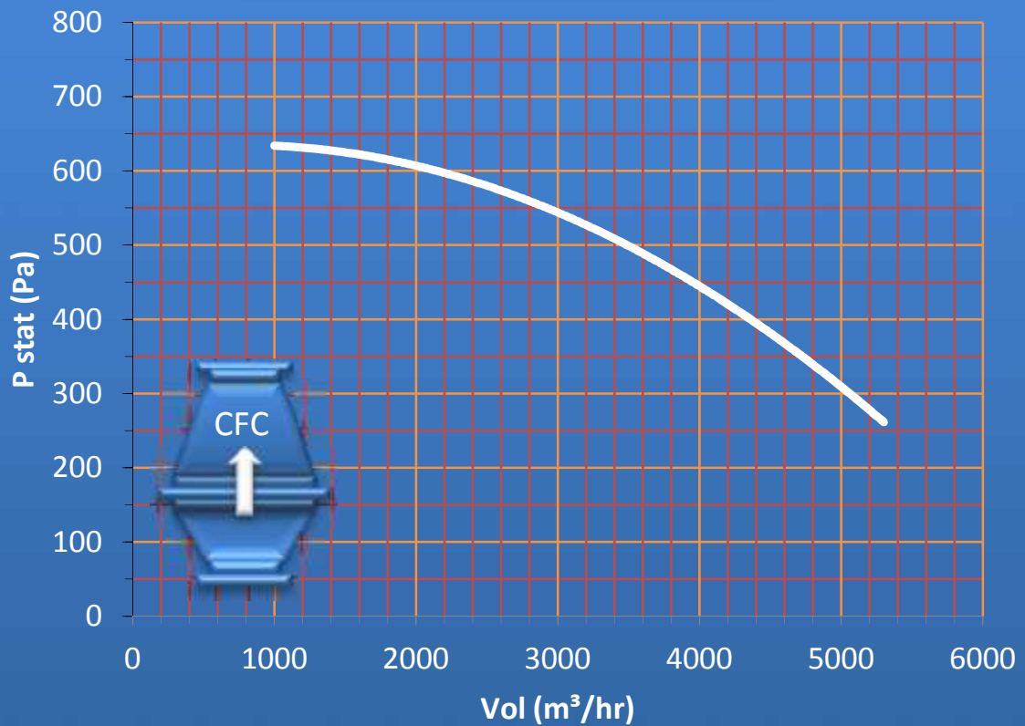
CIV315/315 Performance Curve Motor 2.2kW 1420rpm
